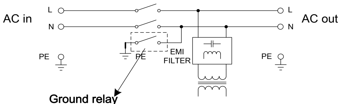
Figure 2-7 Ground Relay Schematic
