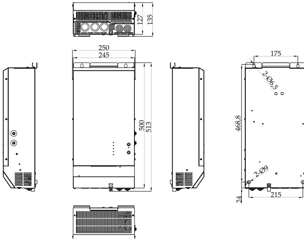
Figure 2-5 Dimension of Bi-directional inverter
